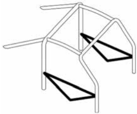
253-10 Door strap drawing
