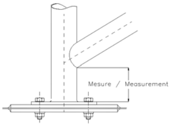
253-52 Drawing showing how screw the fixing plate
