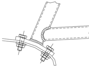
253-57 Drawing showing how screw the fixing plate
