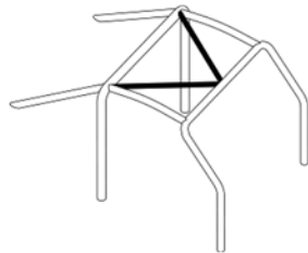
253-13 Drawing of the roof reinforcement
