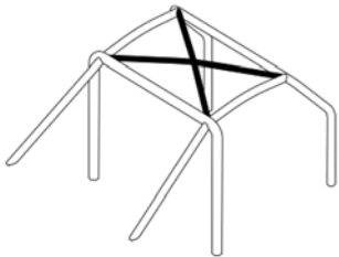
253-12 Drawing of the roof reinforcement
