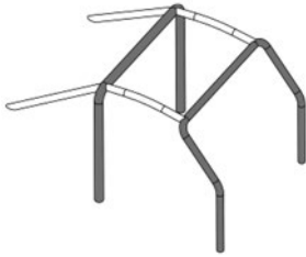
253-3 Basic Cage Drawing
