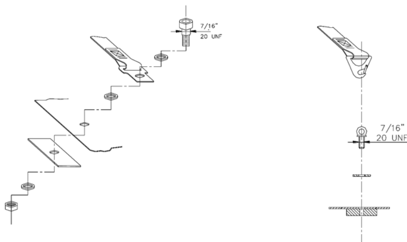
Drawing of the fixing points of the safety belts
