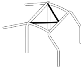
253-13 Drawing of the roof reinforcement
