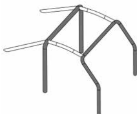
253-3 Basic Cage Drawing
